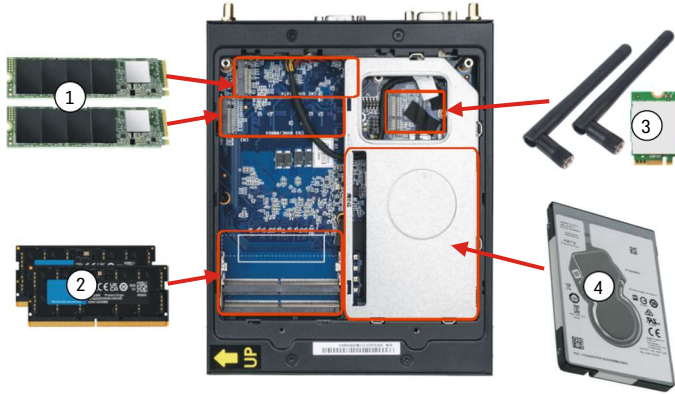
Shuttle XPC slim Barebone DS50U7 with opened chassis
